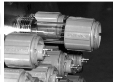
Compression nut assembled on the quartz sleeve
