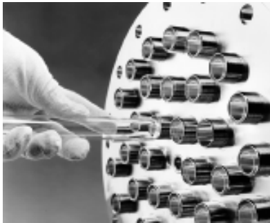
Quartz sleeve installation
