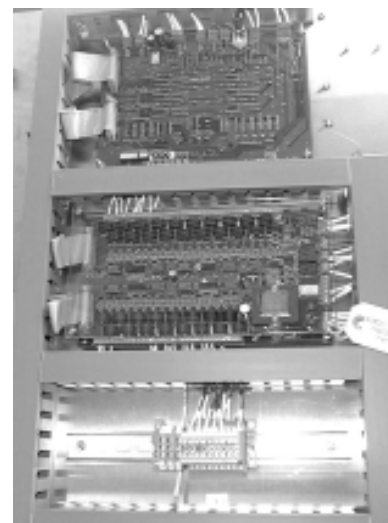
Top item - Status Display Board (SDB) Bottom item - Current Sensing Board (CSB)
