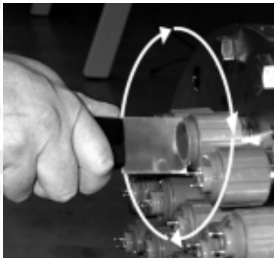
Rotate compression nut clockwise onto the threaded stainless nipped end plate with compression nut tool
