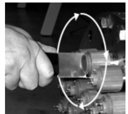
Rotate compression nut clockwise onto the threaded stainless nipped end plate with compression nut tool
